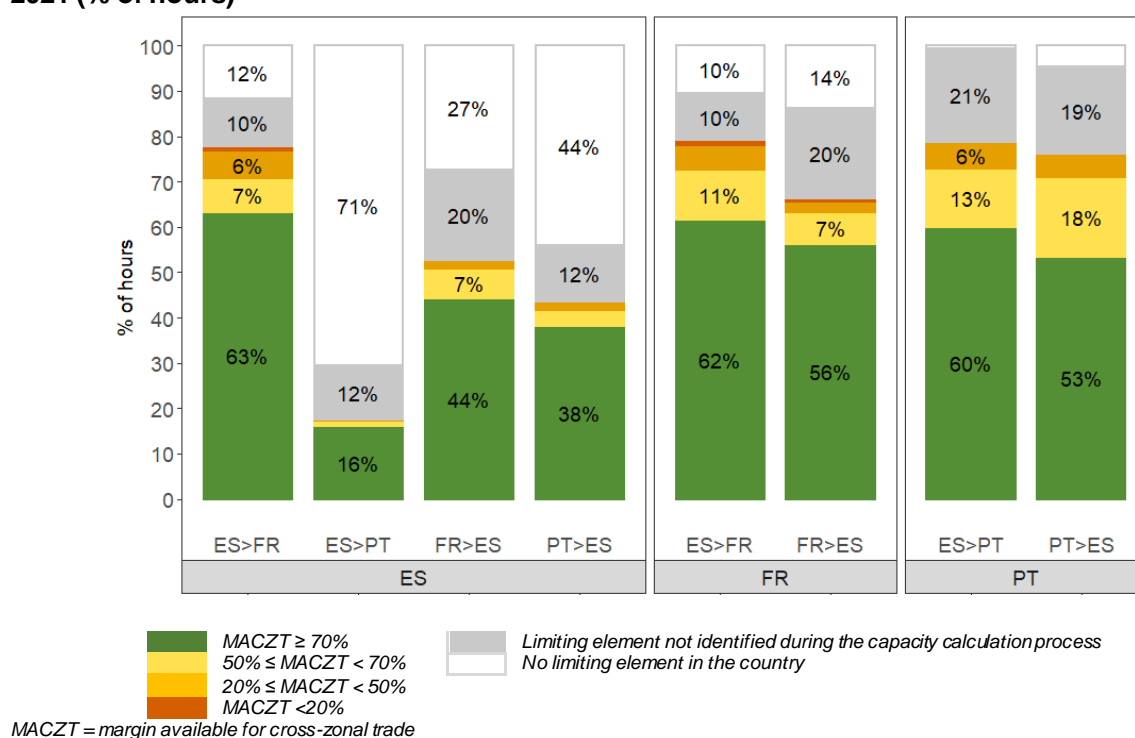
Figure 4: Percentage of the time when the minimum 70% target was reached in the SWE region – 2021 (% of hours)
