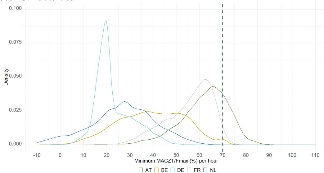
Figure 7: Density function of the lowest hourly relative MACZT per country, in the CWE region – 2021
