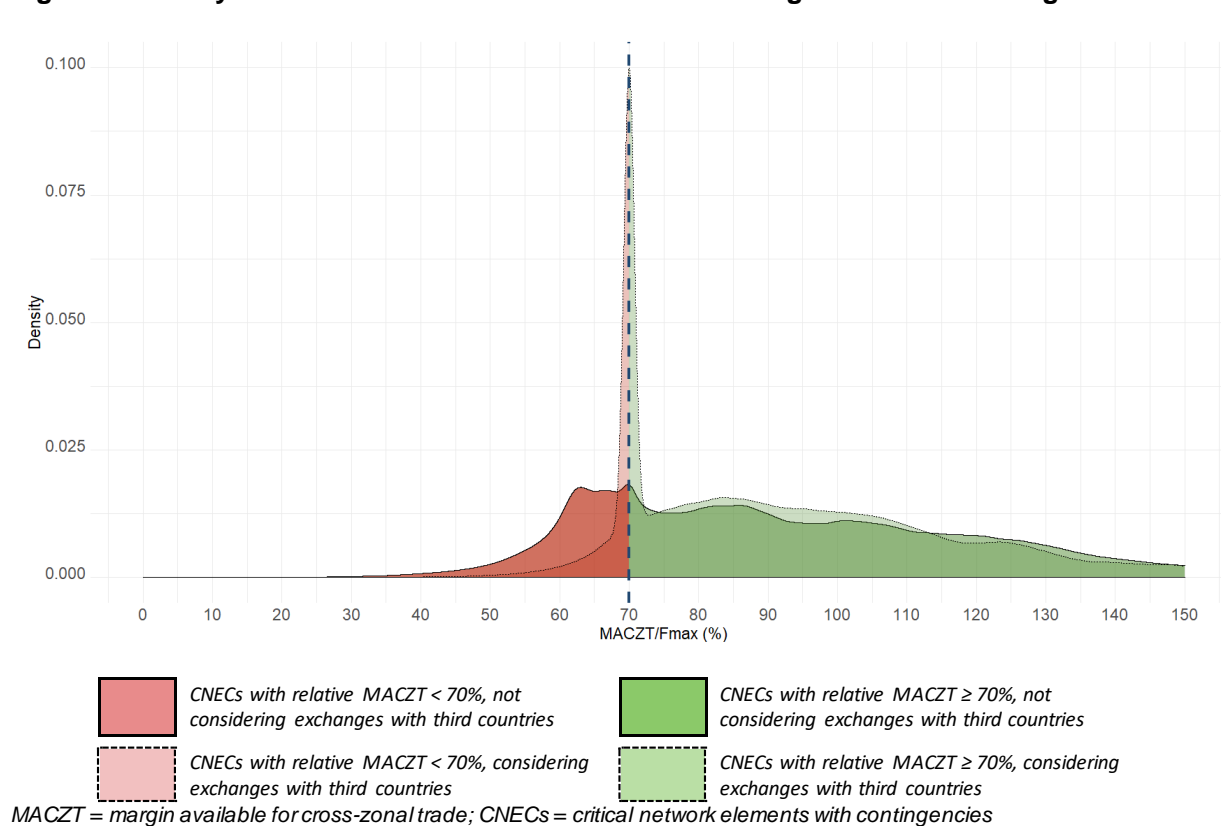
Figure 9: Density function of the MACZT for all CNECs in Belgium for the CWE region – 2021
