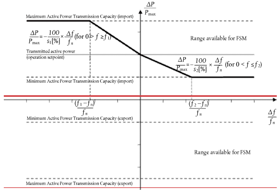
Figure 1: Active power frequency response capability of an HVDC system in FSM illustrating the case of zero with deadband and insensitivity with a positive active power setpoint (import mode) . In this figure, \Delta P is the change in change by an HVDC system with the network at its connection point based on its actual operating point , P_{\max} is maximum transmission capacity of the HVDC system , f_n is the target frequency in the AC network where the FSM service is provided, and \Delta f is the frequency deviation in the AC network where the FSM service is provided, \Delta P_1 is the agreed power change for the FSM at reaching the frequency threshold value \Delta f_1 , \Delta P_2 is the agreed power change at reaching the frequency threshold value \Delta f_2 , \Delta f_{\text{db}} is the deadband of the power frequency response, \Delta f_{\text{insensitivity}} is the frequency response insensitivity (or else the permissible tolerance allowed), s_1 is the droop value for the given \Delta P_1 and s_2 is the droop for the given \Delta P_2 .
