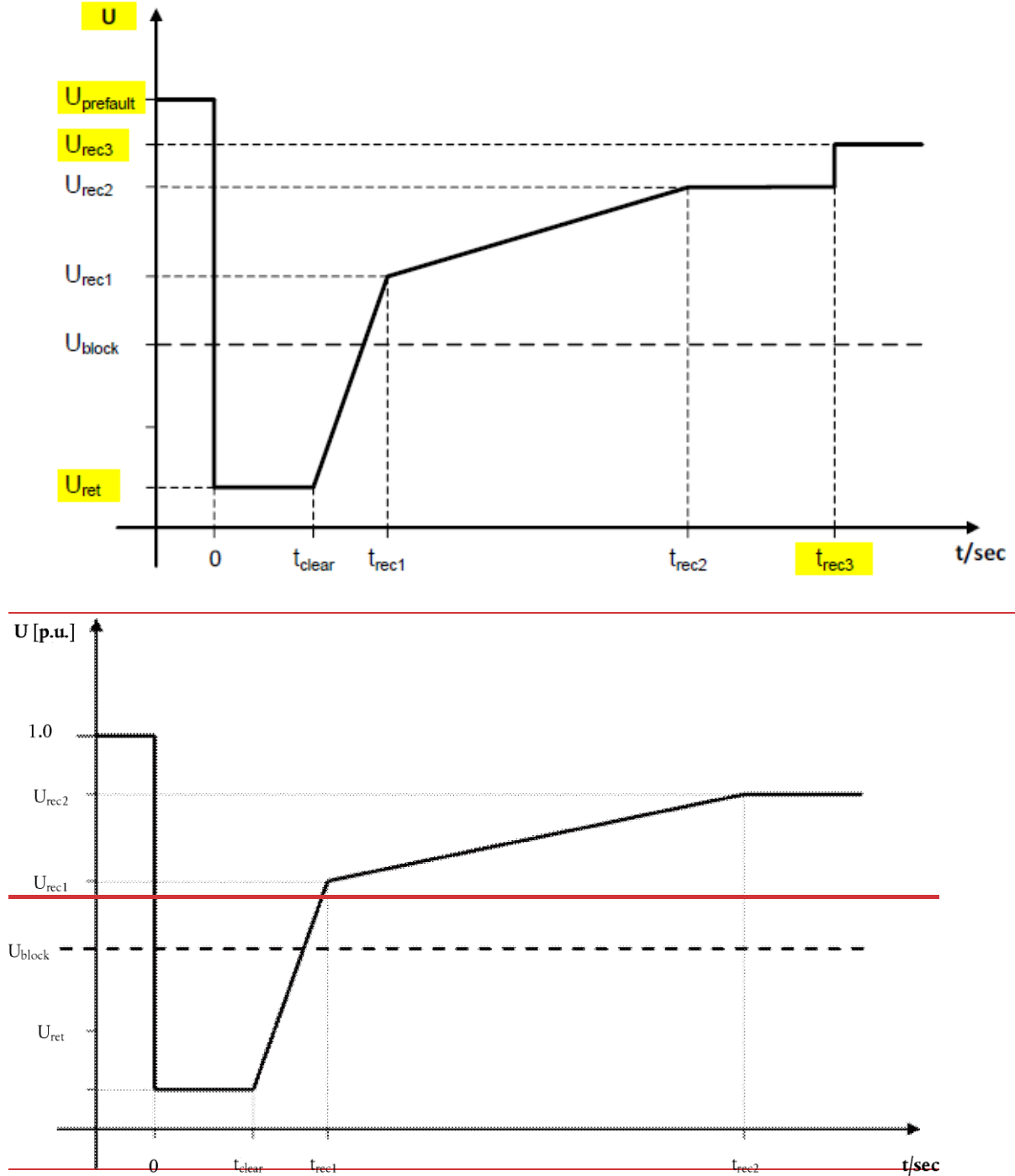
Figure 6: Fault-ride-through Voltage-against-time profile of an HVDC converter station. The diagram represents the lower limit of a voltage- against-time profile at the connection point, expressed by the ratio of its actual value and its reference 1 pu value in per unit before, during and after a fault. U_{\text{prefault}} is the prefault voltage. U_{\text{ret}} is the retained voltage at the connection point during a fault, t_{\text{clear}} is the instant when the fault has been cleared, U_{\text{rec1}} and t_{\text{rec1}} specify a point of lower limits of voltage recovery following fault clearance. U_{\text{block}} is
