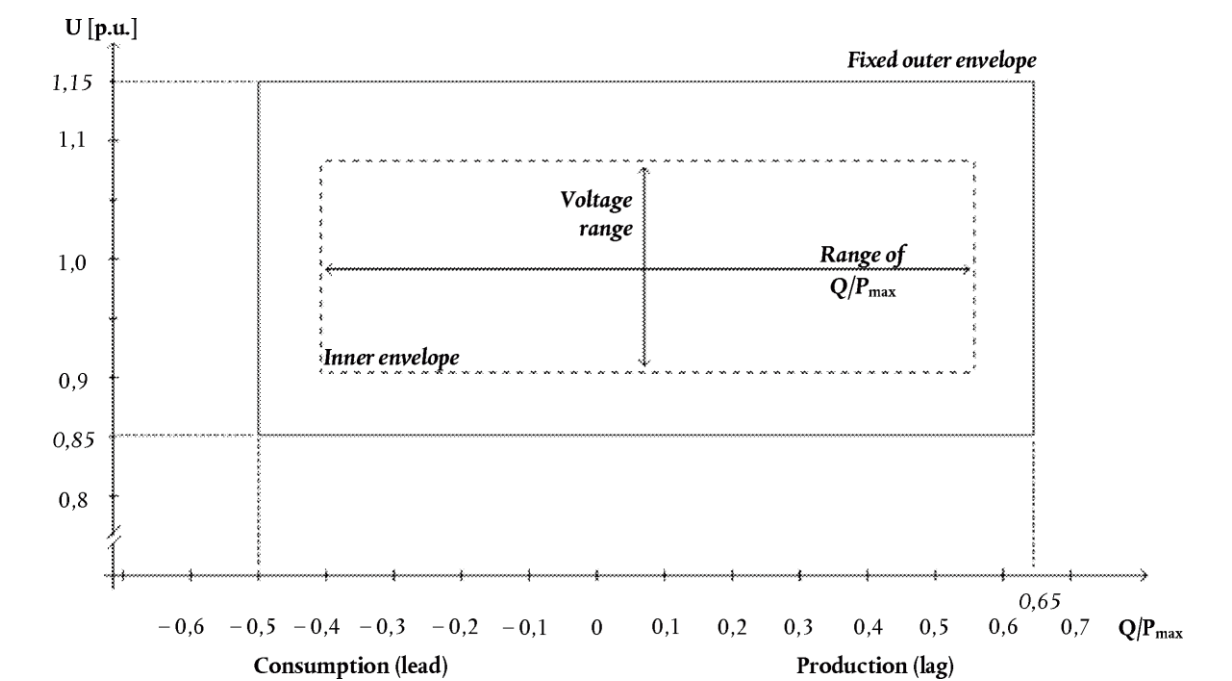
Figure 7: U-Q/P max -profile of an DC-connected power park module A-PPM and A-ESM at the connection point. The diagram represents boundaries of a U-Q/P max -profile of the voltage at the connection point[s], expressed by the ratio of its actual value to its reference 1 pu value in per unit, against the ratio of the reactive power (Q) to the maximum capacity (P max ). The position, size and shape of the inner envelope are indicative and other than rectangular may be used within the inner-fixed outer envelope. For profile shapes other than rectangular, the voltage range represents the highest and lowest voltage points. Such a profile would not give rise to the full reactive power range being available across the range of steady-state voltages.
